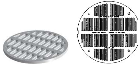
Type M Flat Grate Approx. 360 sq. in. open area
